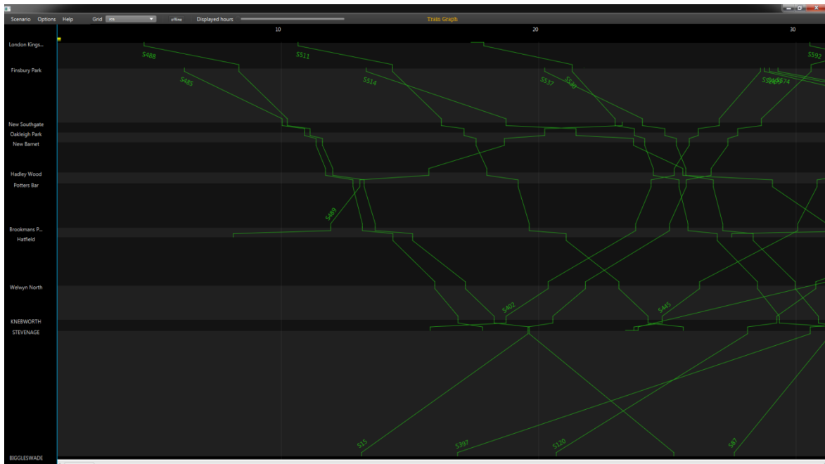
Figure 4-7 - ECML line - Post TMS optimization TG
